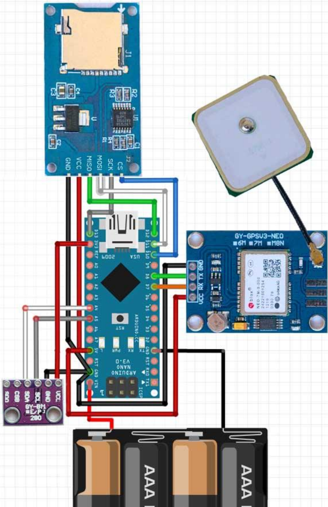
SkyPod wiring diagram
